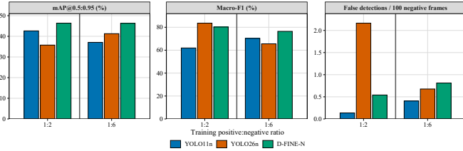
Fig. 4. Six completed NIR protected-test results at seed 13 and deterministic 1-FPS midpoint sampling. Grouped columns compare each completed model at 1:2 and 1:6 training exposures; the dark-grey rule separates the ratio sections. RTMDet-Tiny and EfficientDet-D1 remain pending.
