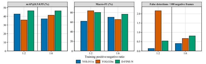
Fig. 4. Six completed NIR protected-test results at seed 13 and deterministic 1-FPS midpoint sampling. Grouped columns compare each completed model at 1:2 and 1:6 training exposures; the dark-grey rule separates the ratio sections. RTMDet-Tiny and EfficientDet-D1 remain pending.
