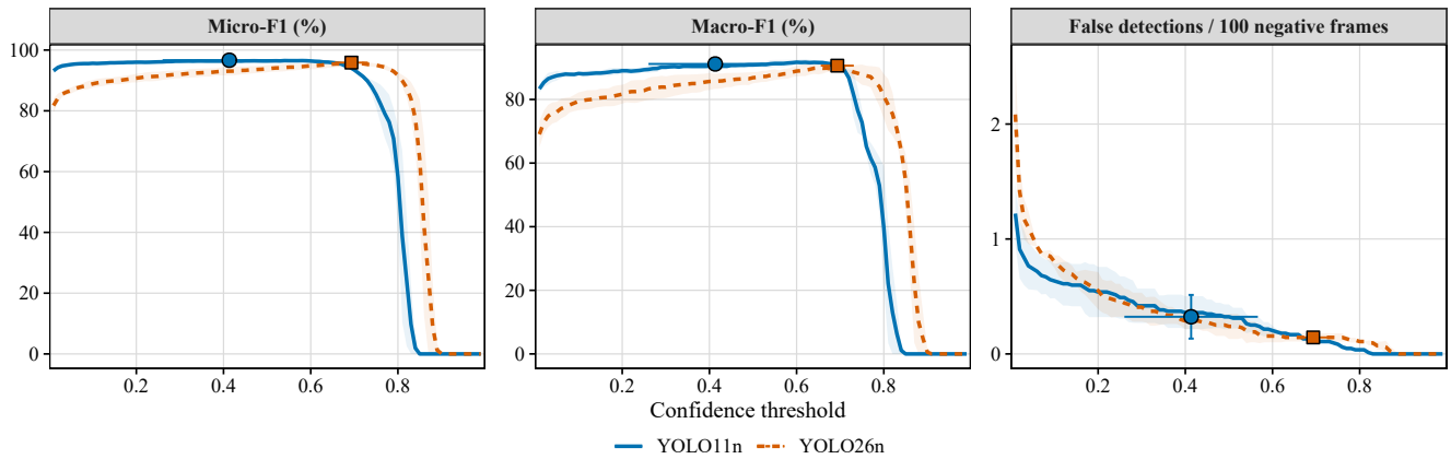
Fig. 4. RGB validation confidence sweep. Lines show the seed mean and light ribbons show sample SD. Each filled marker is the mean micro- F_1 -selected operating point; horizontal and vertical whiskers show the sample SD of its confidence threshold and corresponding metric.
