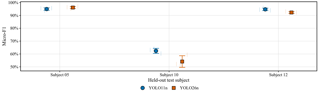
Fig. 3. RGB operating performance by held-out test subject. Pale offset ticks are individual seeds; filled markers and thin error bars show mean \pm sample SD. These bars describe optimization variation on one frozen subject split, not population-level uncertainty across drivers.
