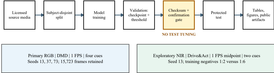
Fig. 1. End-to-end benchmark workflow. RGB and NIR share the validation-before-test gate but retain dataset-specific sampling, ontology, seeds, and training conditions. FPS denotes frames per second. The diagram and all subsequent plots were generated with R/ggplot2.
