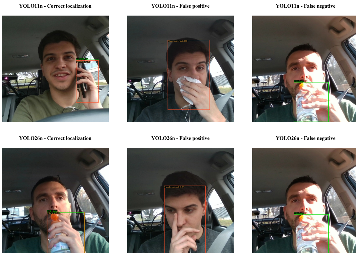
Fig. 5. Representative seed-13 RGB outcomes. Green boxes denote ground truth and orange boxes denote predictions at the validation-selected threshold. Rows are completed detector systems; columns show a true positive, a false detection on a nominal negative, and a false negative.
