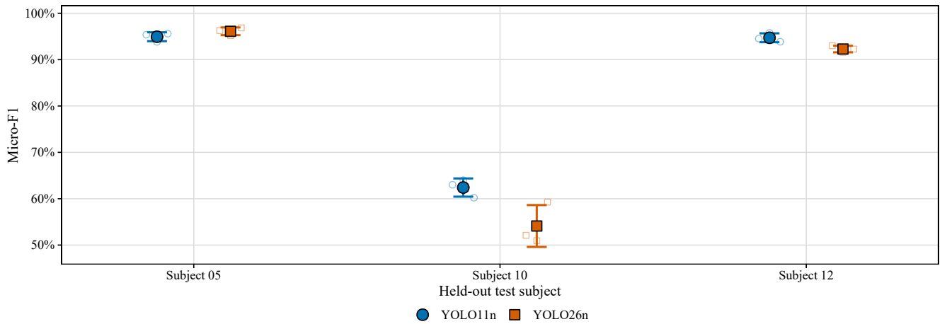
Fig. 3. RGB operating performance by held-out test subject. Pale markers are individual seeds; large markers and error bars show mean \pm sample SD. These bars describe optimization variation on one frozen subject split, not population-level uncertainty across drivers.
