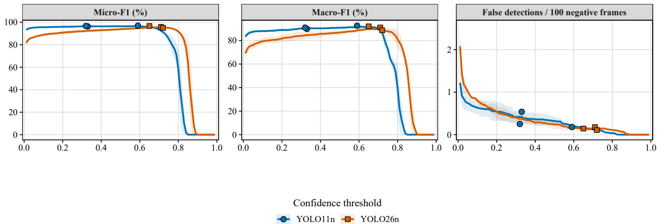
Fig. 4. RGB validation confidence sweep. Lines show the mean and ribbons show sample SD over seeds. Outlined markers identify each seed’s micro- F_1 -selected threshold; they are displayed on all panels only to expose the associated macro- F_1 and false-detection cost.
