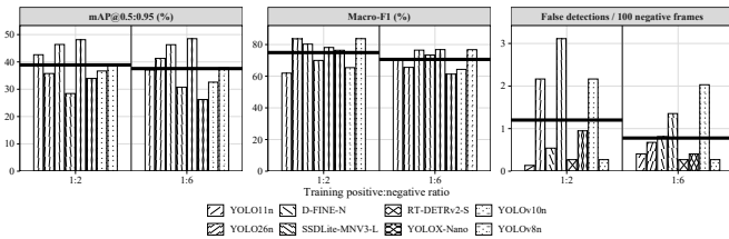
Fig. 4. Sixteen NIR protected-test results at seed 13 and deterministic 1-FPS midpoint sampling. Distinct black-and-white hatch patterns identify the eight models at 1:2 and 1:6 training exposures; the dark-grey rule separates the ratio sections, and each thick black segment marks the eight-model mean for its ratio.
