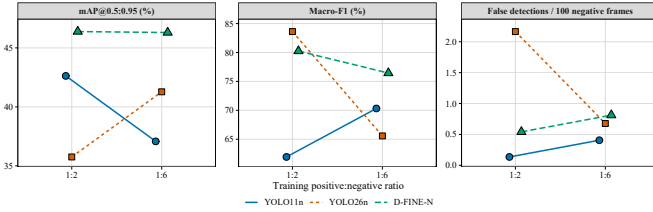
Fig. 4. Six completed NIR protected-test results at seed 13 and deterministic 1-FPS midpoint sampling. Lines connect each completed model's 1:2 and 1:6 training exposures; RTMDet-Tiny and EfficientDet-D1 remain pending.
