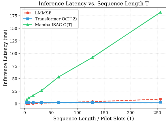
Fig. 5. Inference Latency vs Sequence Length ( T_{\text{slots}} \times N_c ). Note that native selective_scan_cuda is required for Mamba to achieve the depicted theoretical linear baseline advantage in practice.
