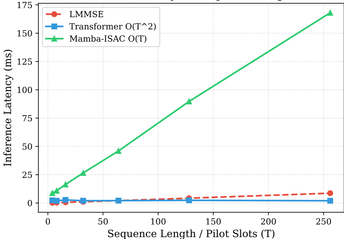
Inference Latency vs. Sequence Length T
