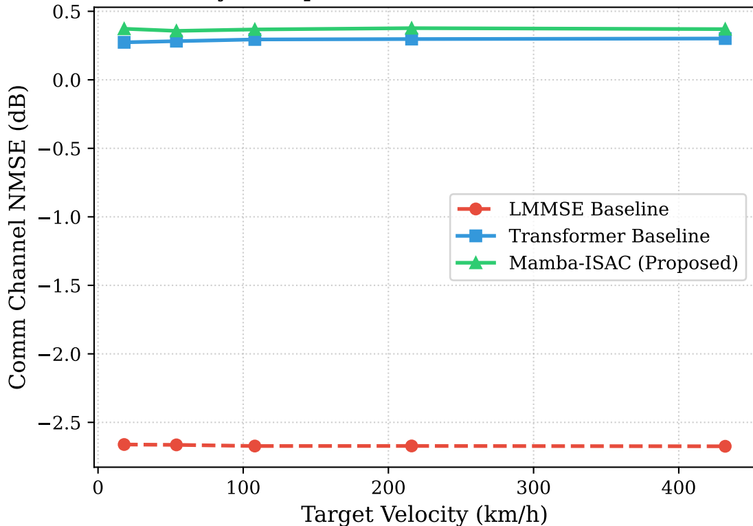
Mobility Sweep: Channel Estimation Robustness
