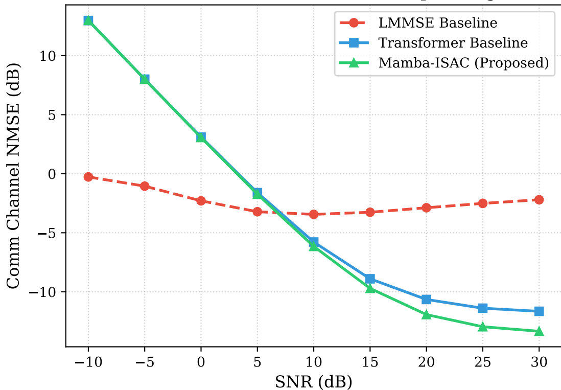
Communication Channel NMSE vs. Operating SNR
