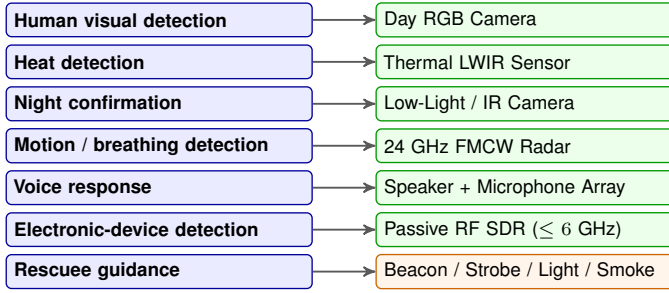
Fig. 3. Operational SAR capability to payload sensor and signaling subsystem mapping.
