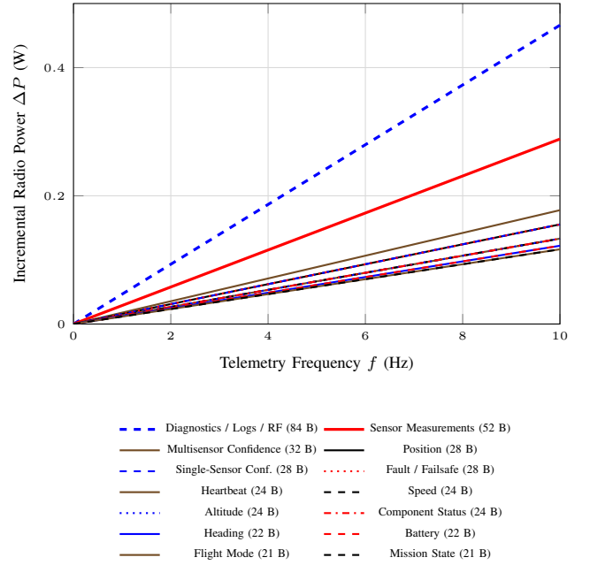
Fig. 6. Analytical estimate of incremental radio power for individual MANAR telemetry message types across transmission frequencies ( P_{TX} = 4.8 W, P_{RX} = 0.36 W, R = 64 kbps).
