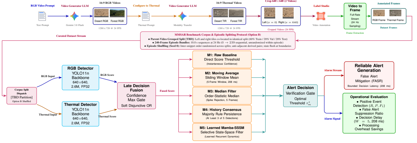
Fig. 1. System architecture of the proposed Multimodal Search and Rescue (MMSAR) evaluation framework. Visible RGB and thermal infrared video streams are synthesized from text prompts and Gemini video generation, followed by cross-modality thermal transfer, dual-crop ( 640 \times 640 ) spatial extraction into left and right viewports, video-level bounding-box annotation in Label Studio, and full-rate 24 Hz frame extraction. Curated sequences are partitioned into 240-frame episodes under a parent-video grouped split protocol (Option B, [TBD]) with anti-adjacency snippet shuffling to eliminate cross-tile spatial leakage. At the edge inference stage, parallel lightweight YOLO11n backbones process incoming RGB and thermal frames at 24 Hz ( T_s \approx 41.7 ms), integrated via soft disjunctive late fusion ( s[n] = \max(c_{\text{RGB}}[n], c_{\text{Thermal}}[n]) ) and evaluated across five lightweight temporal decision methods ( W = 5 frames, 208 ms latency bound). Alert decisions are benchmarked across positive event detection, false alert mitigation, decision delay, and edge processing overhead savings.
