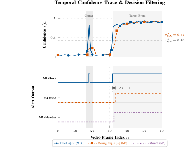
Fig. 2. Temporal sequence trace: (top) fused confidence s[n] with clutter spike at frame 18 and target event from frame 32; (bottom) causal decisions for M1 (spurious alert), M2 (spike suppressed), and M5.
