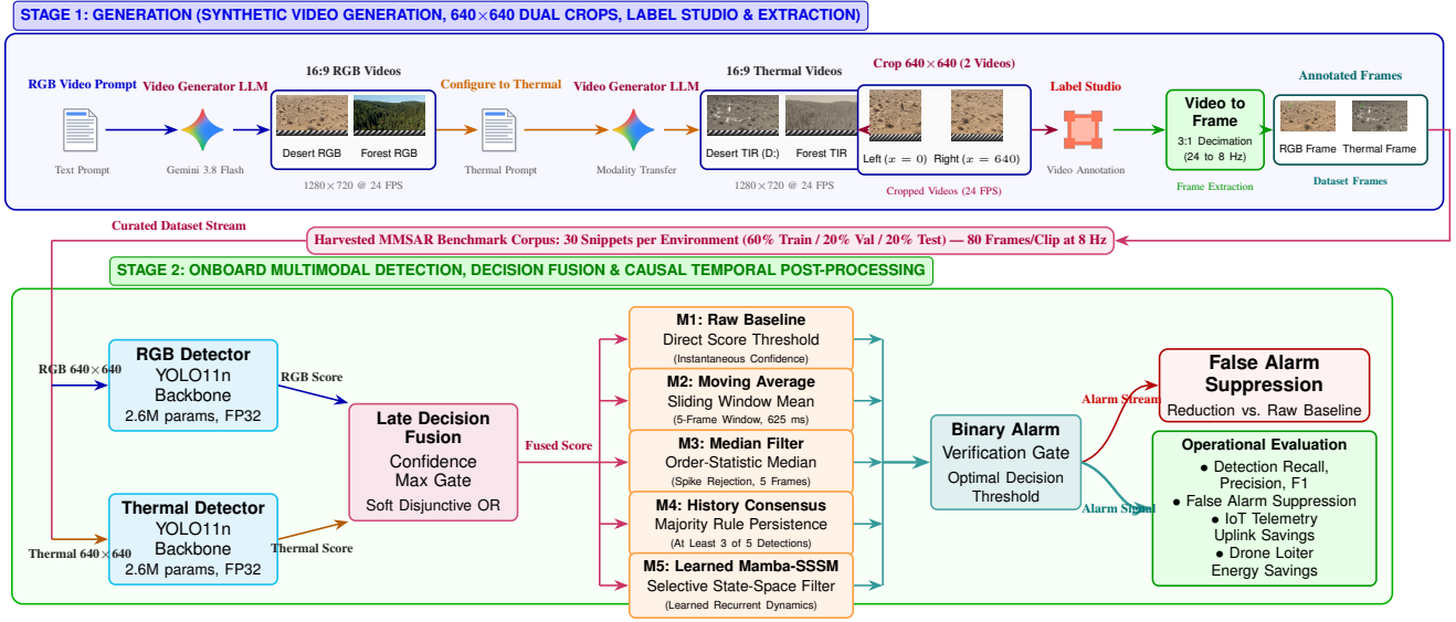
Fig. 1. System architecture of the proposed Multimodal Search and Rescue (MMSAR) evaluation framework. Synchronized RGB and thermal streams (illustrated via the 4 \times 2 environment gallery across desert and forest biomes) are decimated to an 8 Hz timebase ( T_s = 125 ms) and processed by parallel lightweight YOLO11n backbones (one RGB model and one thermal model). Confidence streams are integrated via soft disjunctive late fusion s[n] = \max(c_{\text{RGB}}[n], c_{\text{Thermal}}[n]) and distributed across five competing causal temporal post-processing methods ( W = 5 frames / 625 ms latency bound). Binary alarms are asserted against validation-optimized thresholds \tau_m^* and evaluated across detection reliability and resource overhead.
