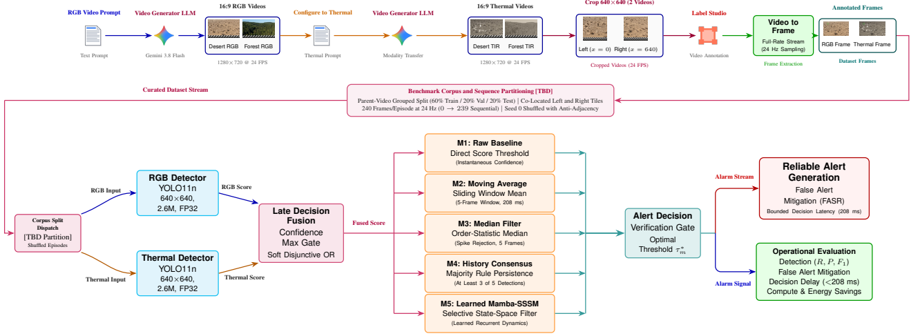
Fig. 1. System architecture of the proposed multimodal search and rescue evaluation framework. Visible RGB and thermal infrared video streams are synthesized from text prompts and Gemini video generation, followed by cross-modality thermal transfer, dual-crop ( 640 \times 640 ) spatial extraction into left and right viewports, video-level annotation in Label Studio, and full-rate 24 Hz frame extraction. Curated sequences are partitioned into 240-frame episodes under a parent-video grouped split protocol (TBD) with anti-adjacency snippet shuffling to eliminate cross-tile spatial leakage. At the edge inference stage, parallel lightweight YOLO11n detectors process incoming RGB and thermal frames at 24 Hz ( T_s \approx 41.7 ms), integrated via soft disjunctive late fusion ( s[n] = \max(c_{\text{RGB}}[n], c_{\text{Thermal}}[n]) ) and evaluated across five lightweight temporal decision methods ( W = 5 frames, 208 ms latency bound). Alert decisions are benchmarked across positive event detection, false alert mitigation, decision delay, and edge processing overhead savings.
