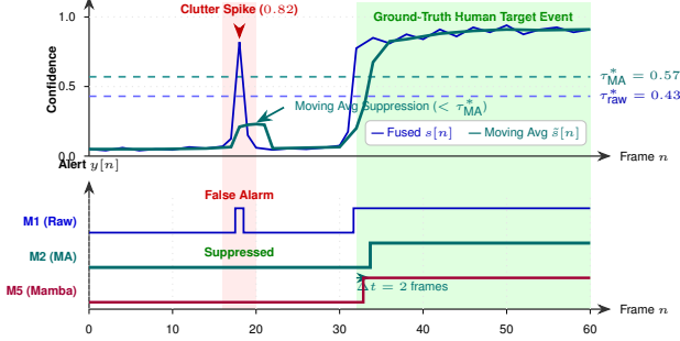
Fig. 2. Temporal sequence trace from an actual held-out test clip: (top) upstream fused confidence s[n] exhibiting an isolated clutter spike at frame 18 followed by a sustained ground-truth target event from frame 32; (bottom) causal binary alert decisions comparing baseline thresholding M1 (spurious alert triggered at frame 18), five-frame moving average M2 (clutter spike completely suppressed, target confirmed with 2-frame latency), and Mamba-SSSM M5.
