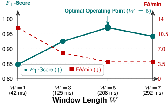
Fig. 3. Temporal window length ablation ( W \in \{1, 3, 5, 7\} ) for the moving average filter on the held-out test split, showing F_1 -score ( \uparrow ) and False Alerts/min ( \downarrow ) across causal latency bounds (42 ms to 292 ms at 24 Hz). W = 5 achieves peak F_1 (0.971) and minimizes false alarms.
