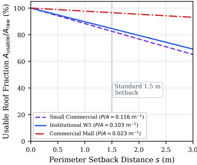
Fig. 6. Usable rooftop area percentage as a function of perimeter setback distance s across three building scales, illustrating the governing influence of the perimeter-to-area ( P/A ) ratio.
