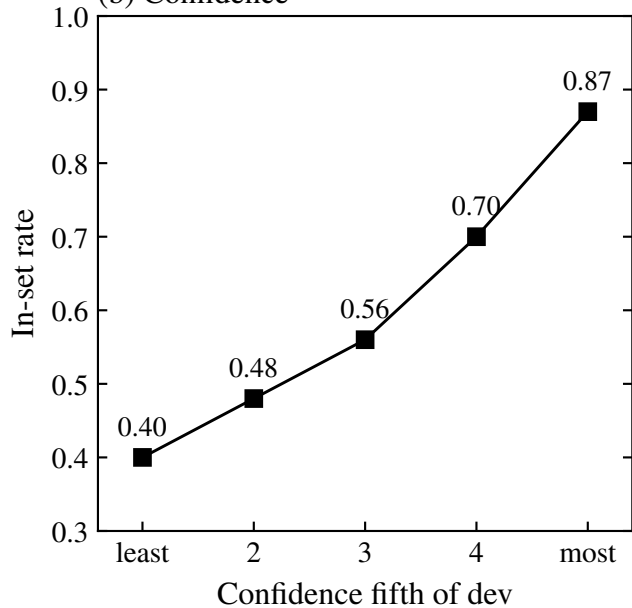
(b) Confidence
