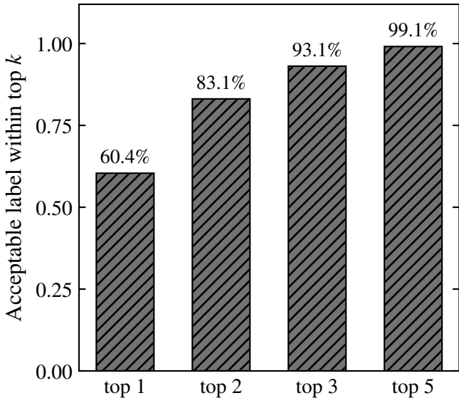
(a) Ranking
