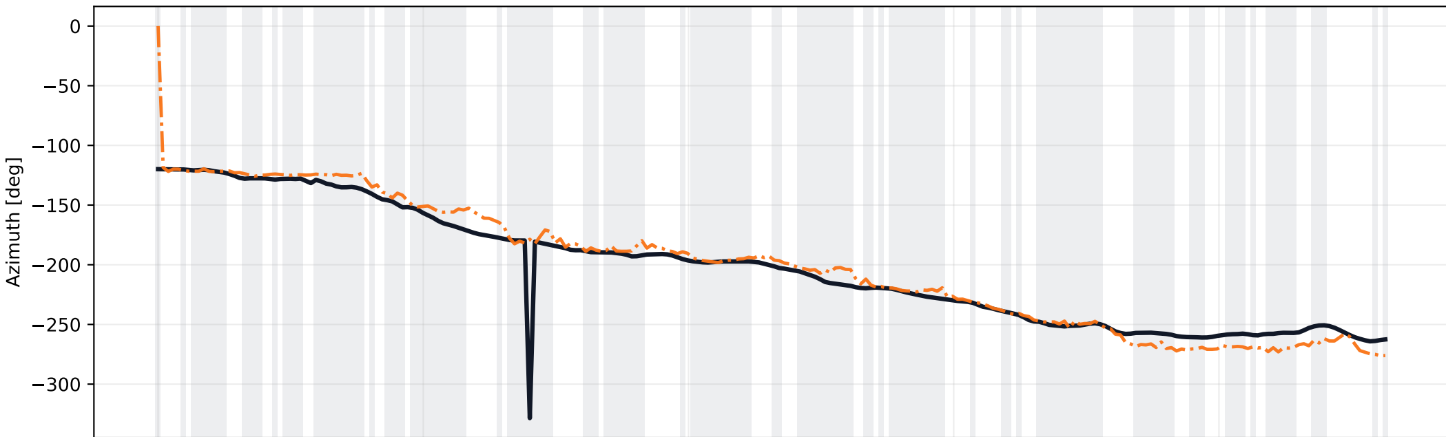
LOCATA eval/task5/recording3/benchmark2 tracking - DFA-IcoNet-Edge
