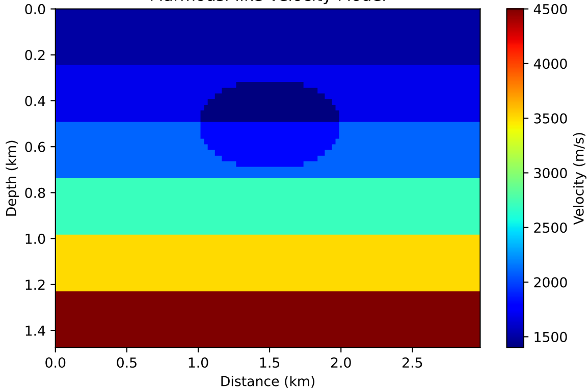
Marmousi-like Velocity Model
