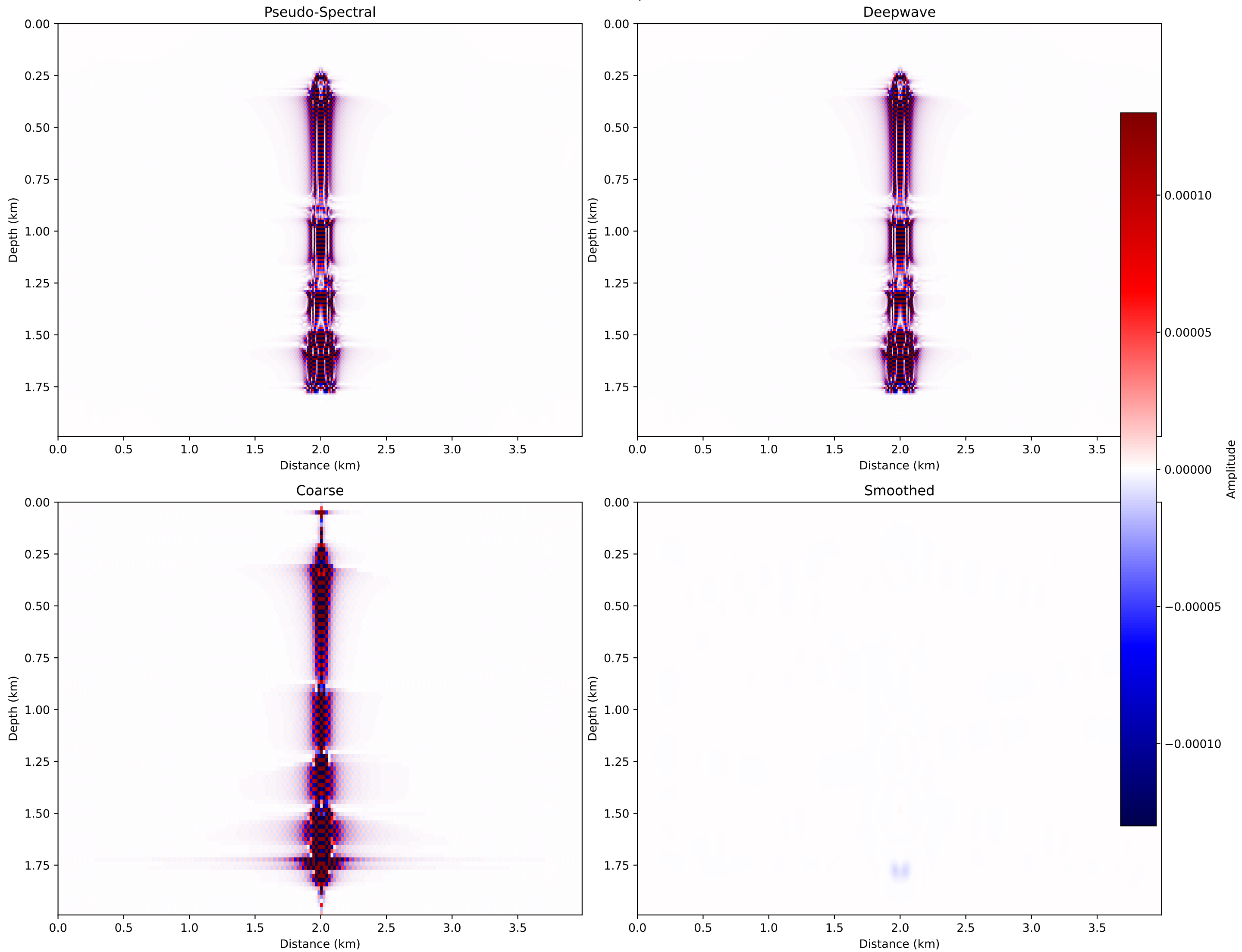
Wavefield Comparison at t = 500 ms
