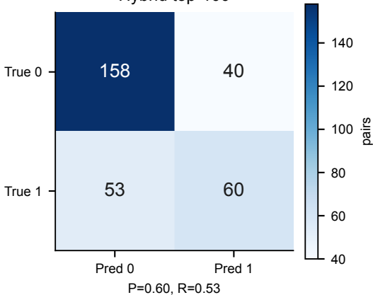
Hybrid top-100
