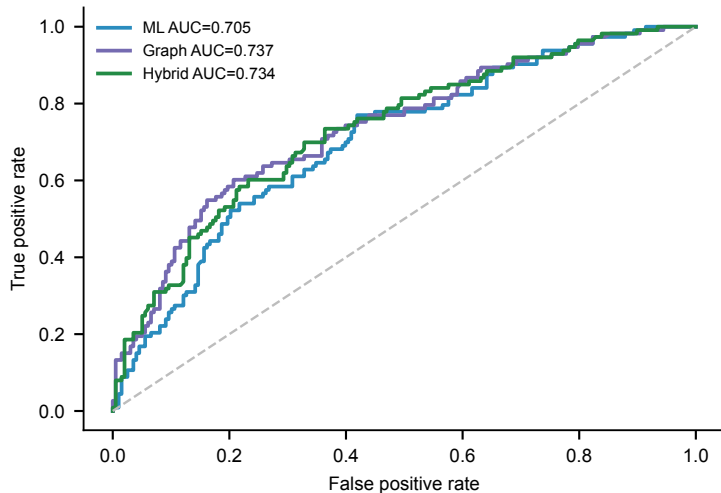
ROC curve
