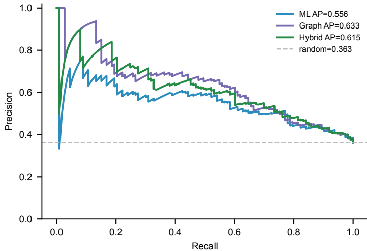
Precision-recall curve
