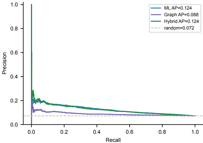
Precision-recall
