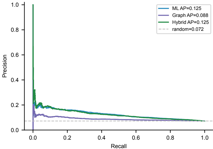
Precision-recall
