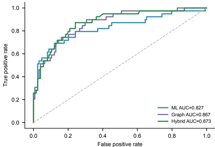
ROC curve
