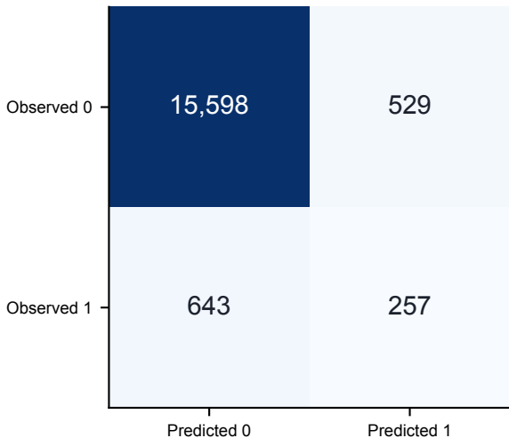
Hybrid confusion matrix rolling-validation threshold=0.914; P=0.327, R=0.286, F1=0.305
