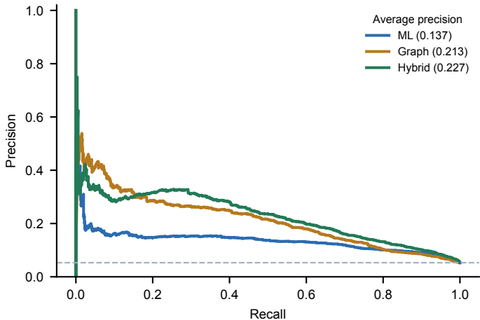
b Precision-recall (baseline = 0.053)
