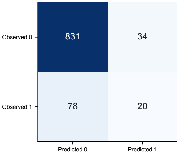
Hybrid confusion matrix rolling-validation threshold=0.842; P=0.370, R=0.204, F1=0.263
