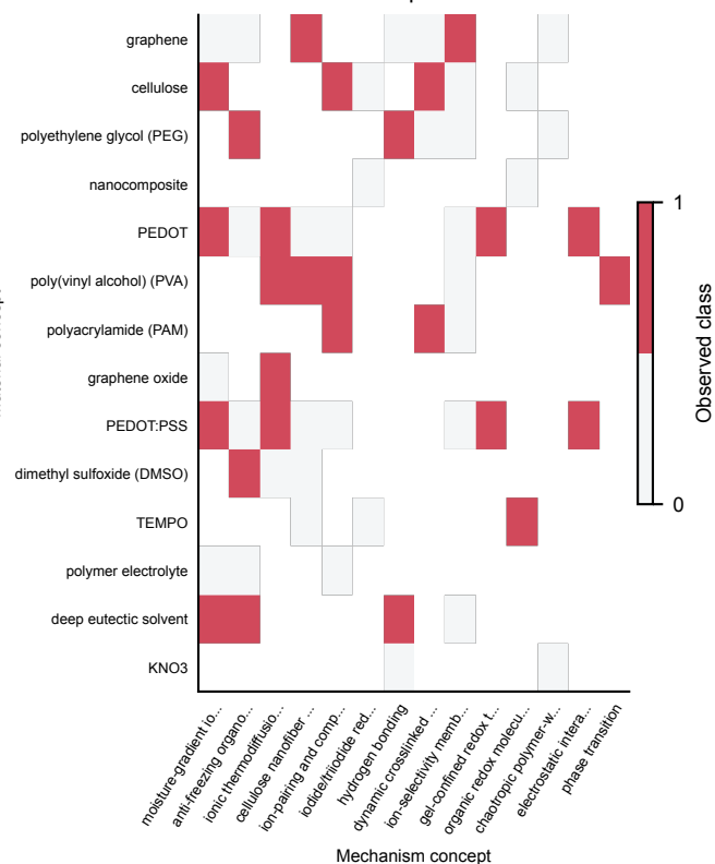
b Observed TG adoption
