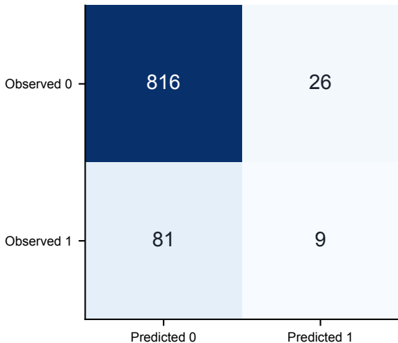
Hybrid confusion matrix rolling-validation threshold=0.899; P=0.257, R=0.100, F1=0.144
