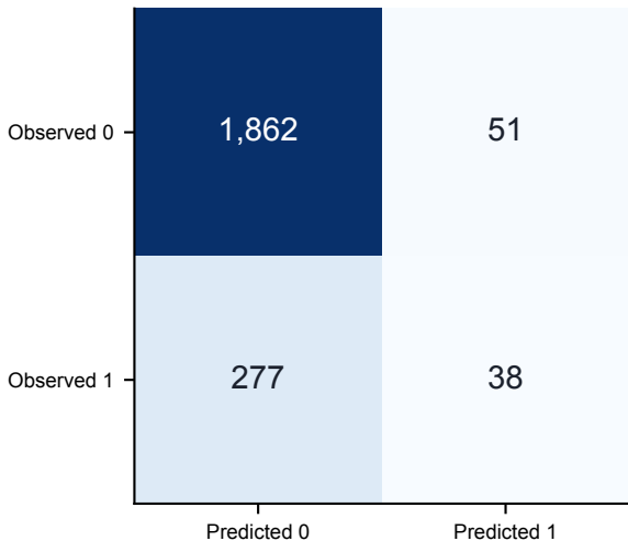
Hybrid confusion matrix rolling-validation threshold=0.912; P=0.427, R=0.121, F1=0.188
