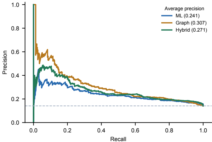
b Precision-recall (baseline = 0.141)
