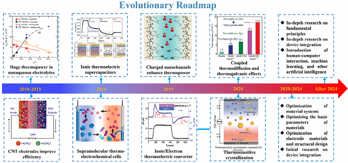
Figure 1.2: Representative evolutionary roadmap of ionic thermoelectrics, adapted from Shang et al. [3].
