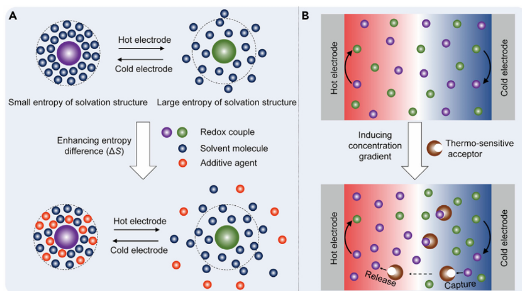
Figure 1.4: Two general routes to higher thermogalvanic thermopower: increasing the solvation-structural entropy difference and inducing a redox concentration gradient. Adapted from Duan et al. [5].
