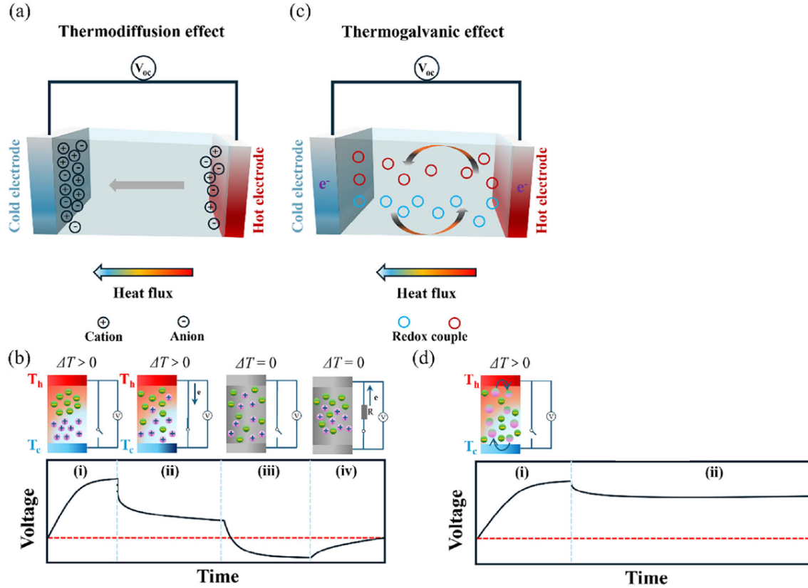
Figure 1.3: Mechanistic distinction between thermodiffusion and thermogalvanic effects in ionic thermoelectric devices, adapted from Lin et al. [7].
