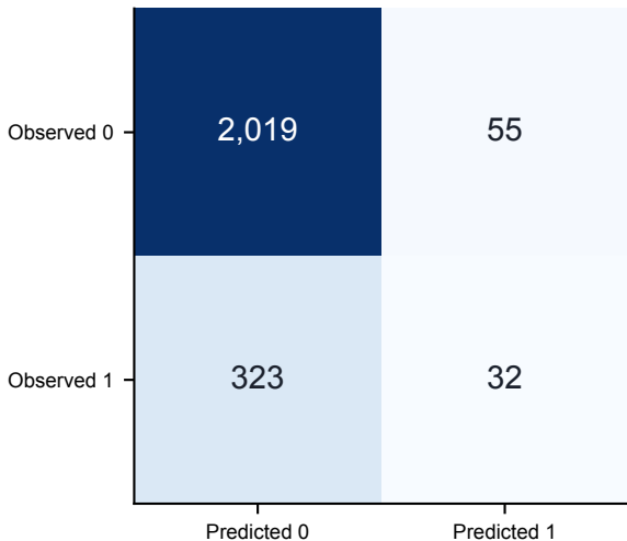
Hybrid confusion matrix rolling-validation threshold=0.915; P=0.368, R=0.090, F1=0.145
