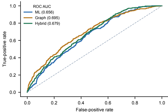
a ROC: new concept-pair classification
