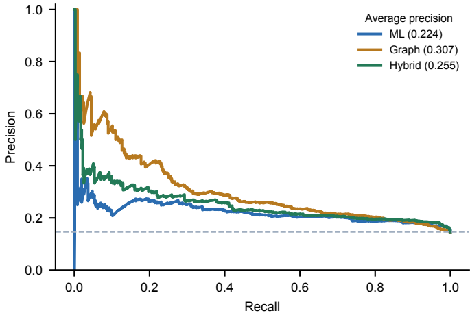
b Precision-recall (baseline = 0.146)
