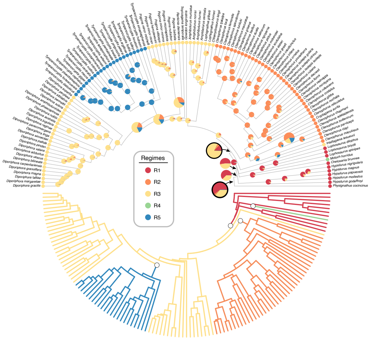
Figure S9. Adaptive peaks corresponding to morphological regimes identified under a multi-optima OU model in PhyloEM and applied to ancestral taxa using randomForests. (Bottom) Tree shows the preferred 5 regime model estimated from all 19 size corrected morphological traits, with regime shifts denoted by small white circles. (Top) Tree shows the preferred 5 regimes including likelihoods for ancestors as estimated by randomForest. The amphibolurine MRCA is estimated as a Hypsilurus / Lophosaurus -like arboreal dragon and the Australian MRCA is estimated as a semiarboreal generalist lizard (both indicated with black outline to pie).
