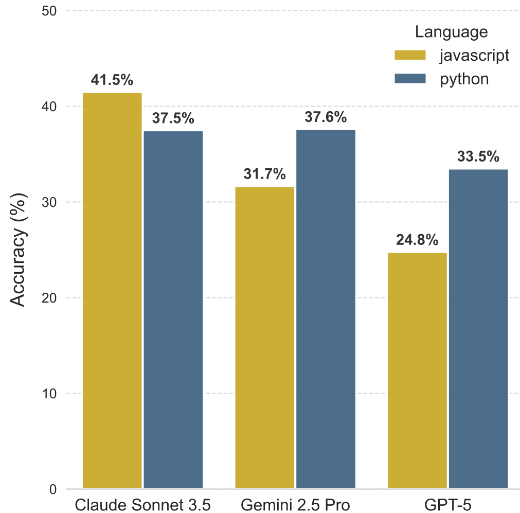
Strict Accuracy: Python vs JavaScript
