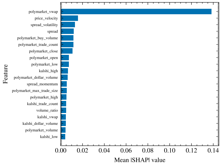
Feature importance (top 20)
