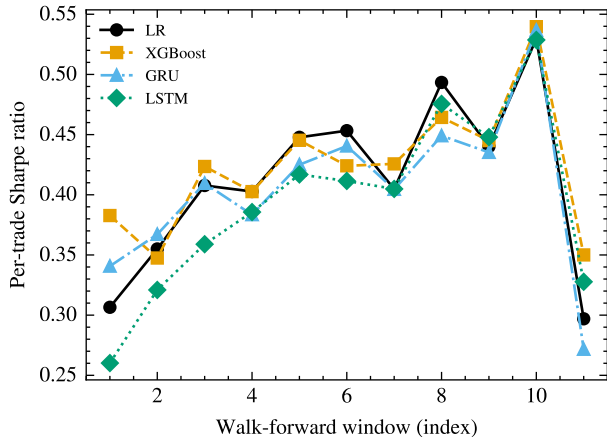
Walk-forward Sharpe trajectory
