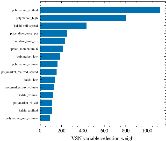
TFT variable-selection weights (top 15)
