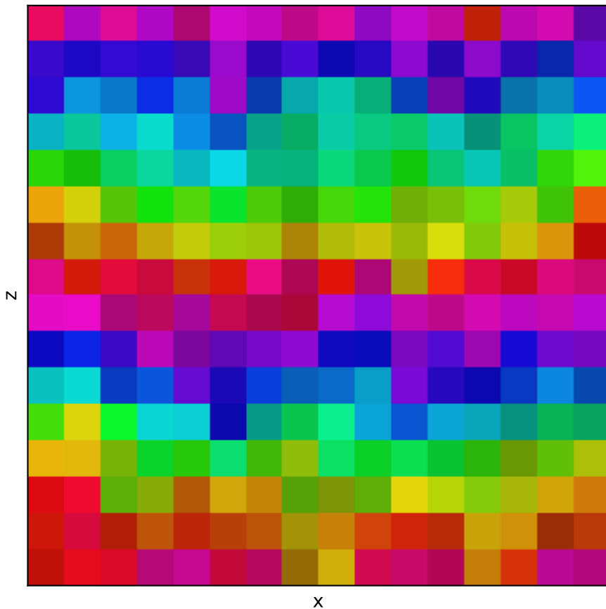
Low T colored xz slice
