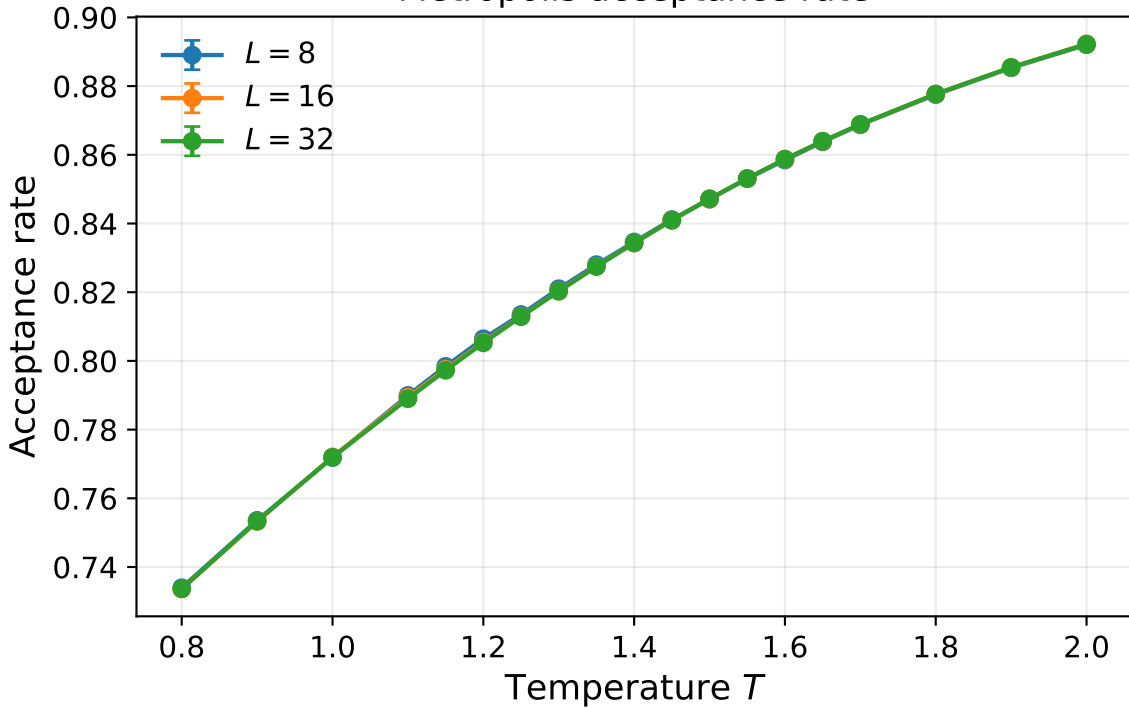
Metropolis acceptance rate
