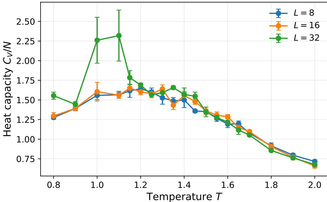
Heat capacity from energy fluctuations
