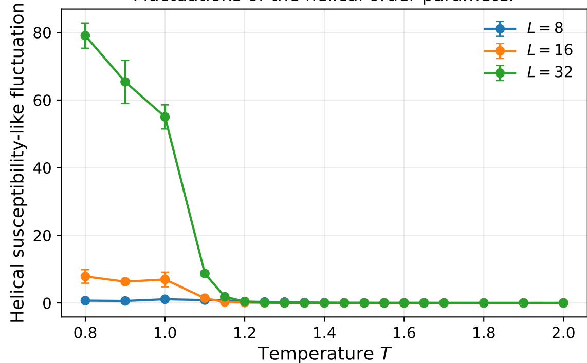
Fluctuations of the helical order parameter
