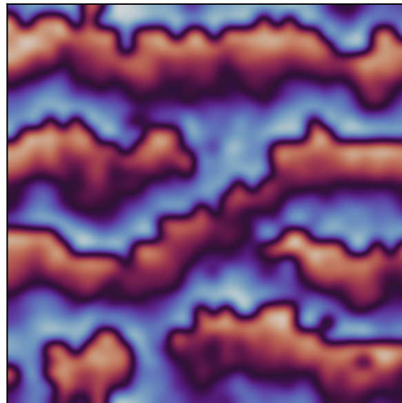
Phase change in colored spin-angle xz slices, L=32
