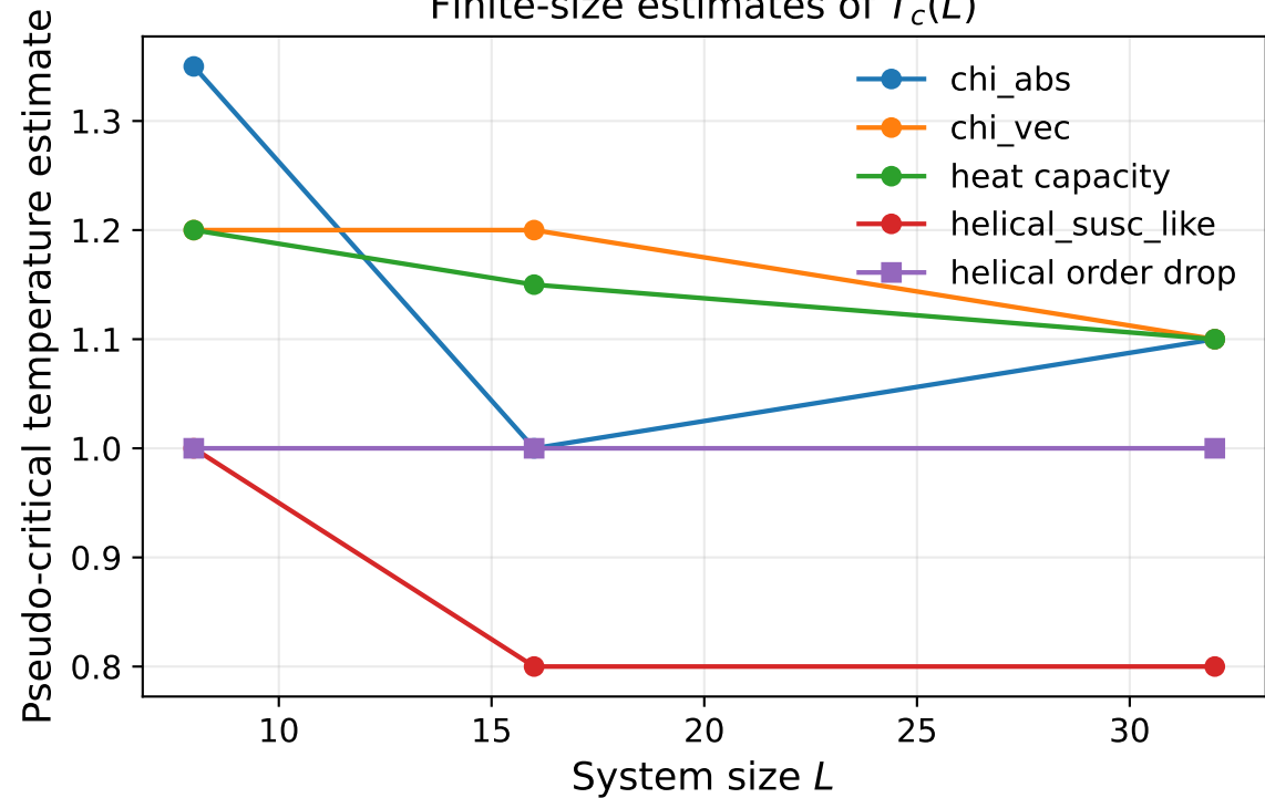
Finite-size estimates of T_c(L)
