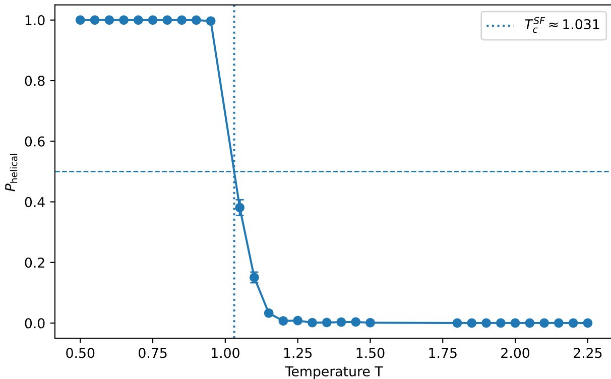
Structure-factor model
