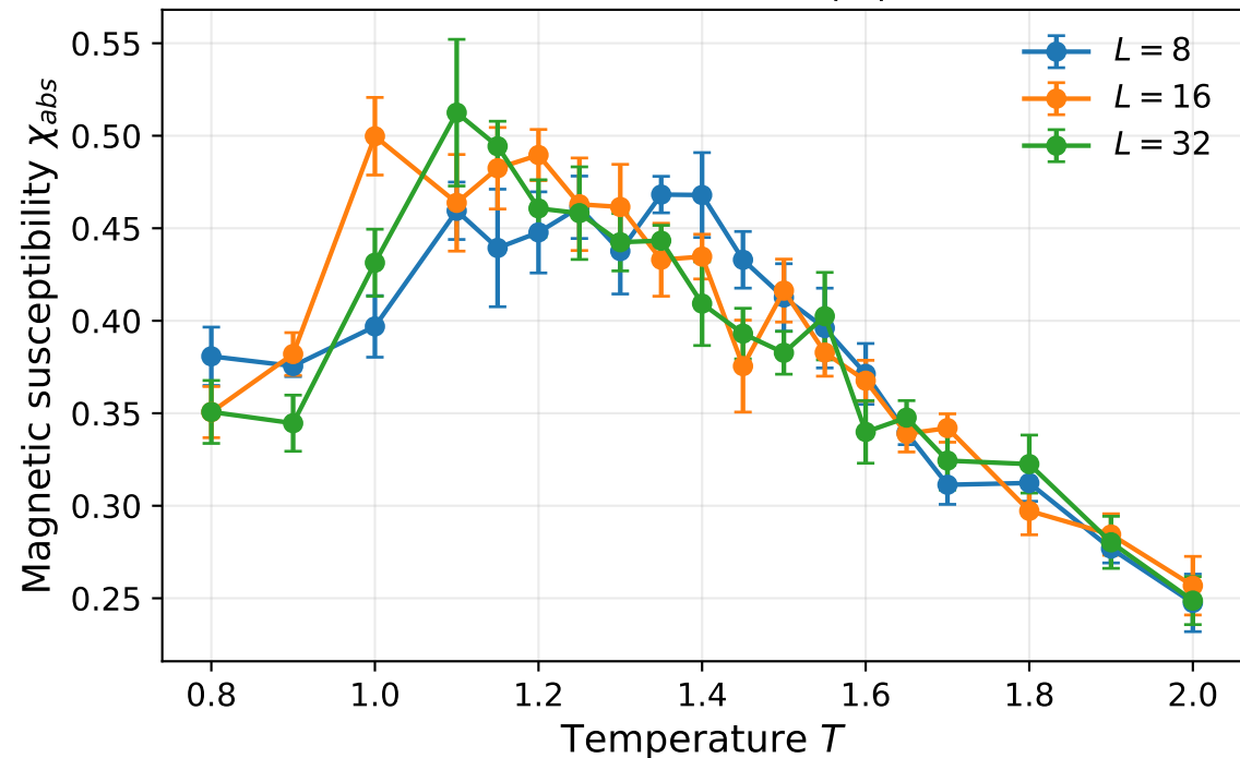
Magnetic susceptibility from |M| fluctuations
